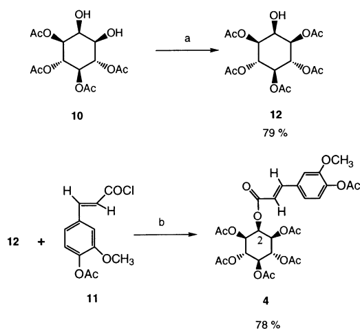
Scheme 1. (a) CH_3COCl , pyridine, DMAP, CH_2Cl_2 , rt; (b) Et_3N , DMAP, CH_2Cl_2 , rt.
