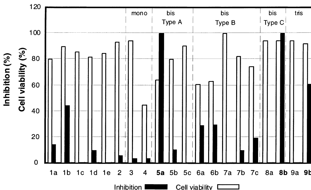
Figure 2. Suppressive effects of feruloyl- myo -inositol derivatives on TPA-induced O 2 - generation in differentiated HL-60 cells. O 2 - generation was induced by TPA (50 nM) and detected by cytochrome c . Sample concentration was 100 μM. Open and closed bars represent cell viability (%) and O 2 - generation suppression (%), respectively. Data are shown as mean values from duplicate experiments.
