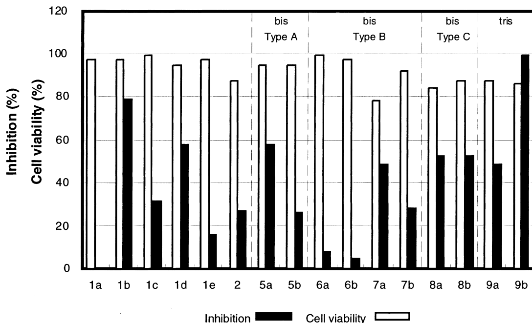
Figure 4. Suppressive effects of feruloyl- myo -inositol derivatives on TPA-linduced EBV activation in Raji cells. Cells were incubated with n -butyric acid (3 mM), TPA (50 nM), and test compound (100 \mu M). EBV activation was measured by detecting early antigen (EA)-induction. Open and closed bars represent cell viability (%) and EBV activation suppression (%), respectively. Data are shown as mean values from duplicate experiments.
