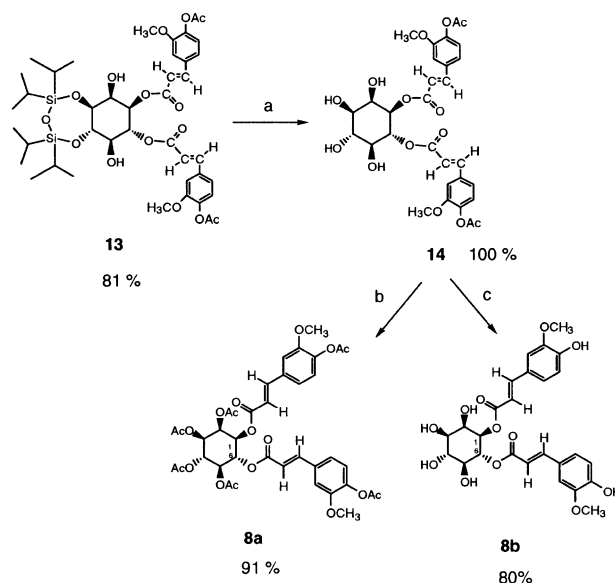
Scheme 3. (a) n-Bu_4NF \cdot 3H_2O , PhCO_2H , THF, -5 to 0 °C; (b) (CH_3CO)_2O , DMAP, pyridine, rt; (c) NH_2NH_2 \cdot H_2O , MeOH, rt.
