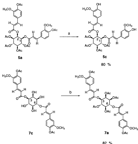
Scheme 2. (a) NH_2NH_2 \cdot H_2O , CHCl_3/MeOH (10:1), rt; (b) (CH_3CO)_2O , pyridine, 90 °C.
