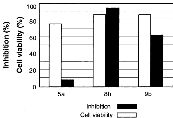
Figure 3. Suppressive effects of feruloyl- myo -inositol derivatives 5a , 8b , and 9b at a concentration of 20 μM. Data are shown as mean values from duplicate experiments.
