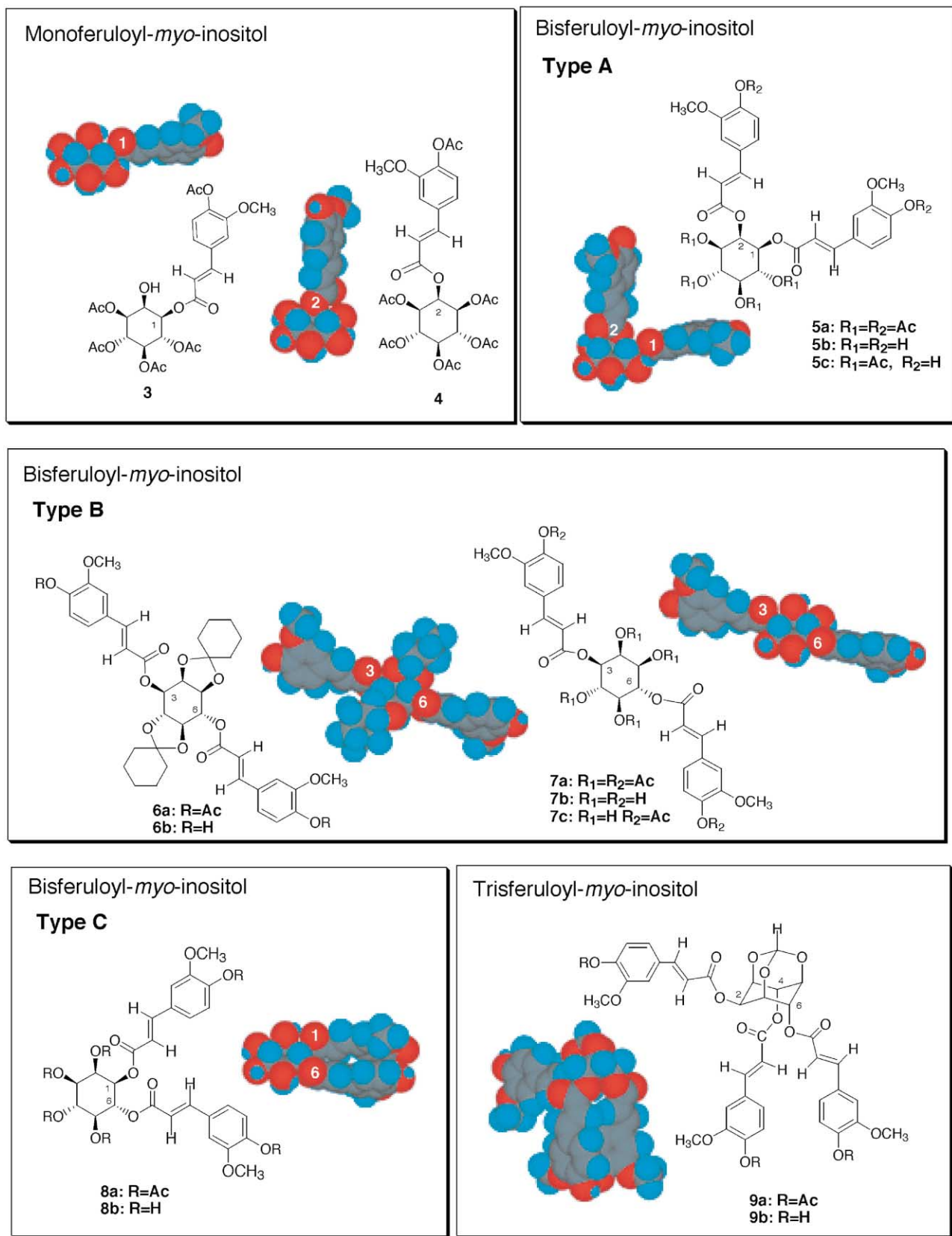
Figure 1. The structure of feruloyl- myo -inositols. Typical stereostructures of the molecules (space-filling model) are provided as the energy-minimized structures.
